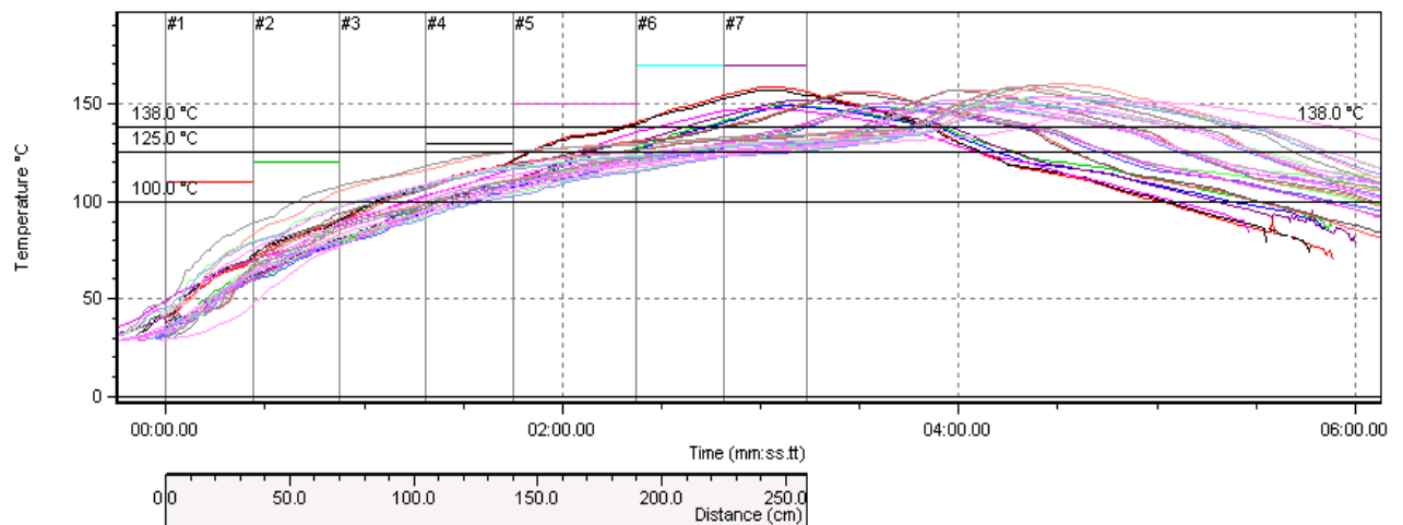
Figure #1 – CVP-520 Reflow Profile Envelope
